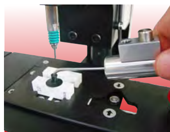
30x9mm Gauge block calibration
